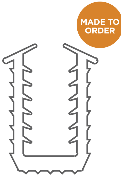
Drawing Number D02778 Part Number 01100024E038 Material EPDM
