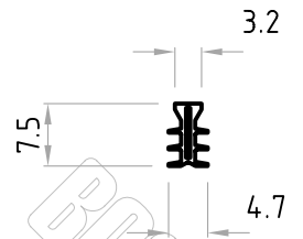
Part No. SK-0675 WITH HARD BACK CENTRE RIB
