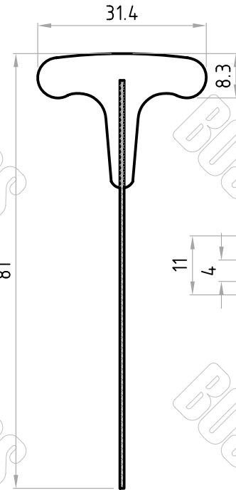
Part No. D02643 WITH FABRIC INSERT
