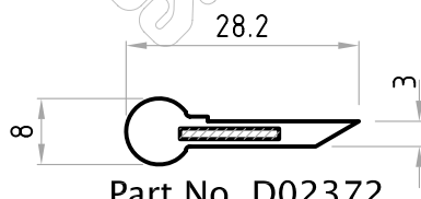
Part No. D02372 WITH HARD BACK INSERT
