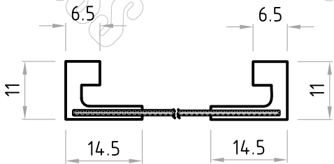
Part No. D00336 WITH FABRIC INSERT
