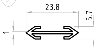
Part No. D02378
