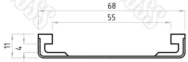
Part No. D03392 WITH FABRIC INSERT
