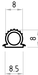
Part No. D03081
