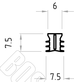
Part No. SK-0675-1 WITH HARD BACK CENTRE RIB
