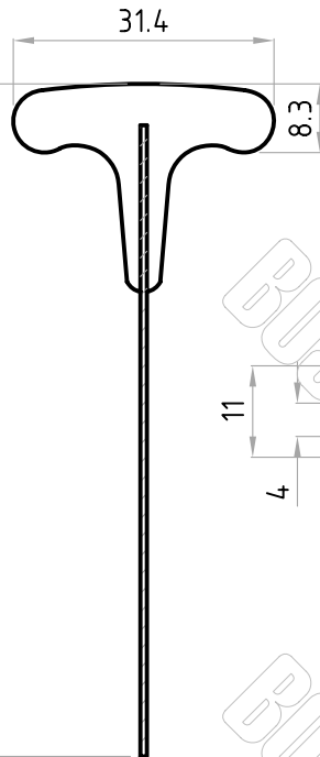
Part No. D02643 WITH FABRIC INSERT
