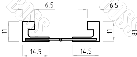
Part No. D00336 WITH FABRIC INSERT
