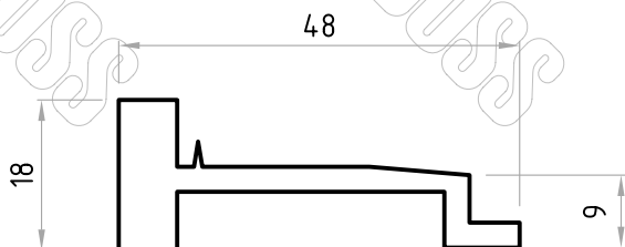
Part No. D02698
