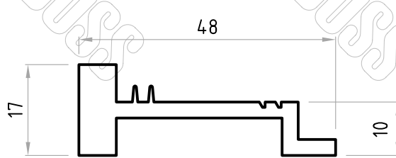
Part No. D02631
