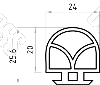
Part No. D02179
