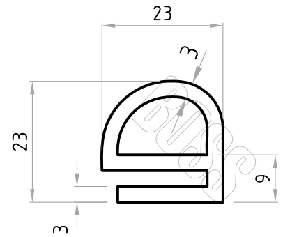
Part No. D02364
