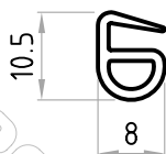
Part No. D03549
