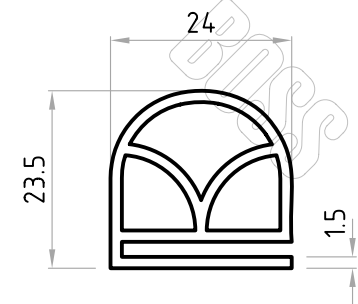
Part No. D02178
