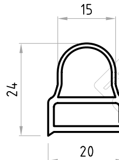
Part No. D02280
