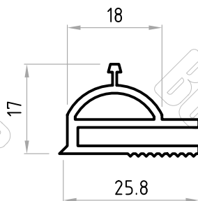
Part No. D02265
