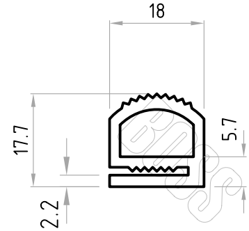
Part No. D01096
