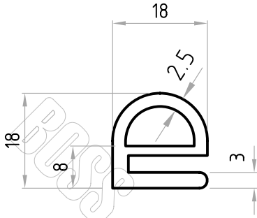
Part No. D00586
