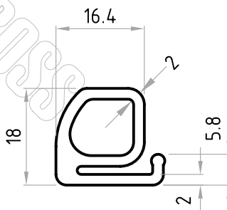
Part No. D02520
