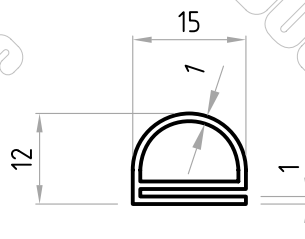
Part No. D02685
