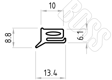
Part No. D03049
