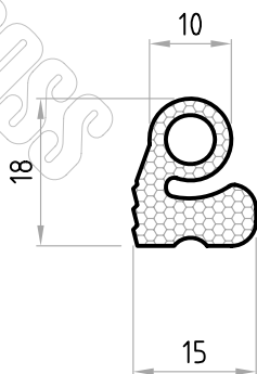
Part No. D02217
