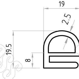
Part No. D00587
